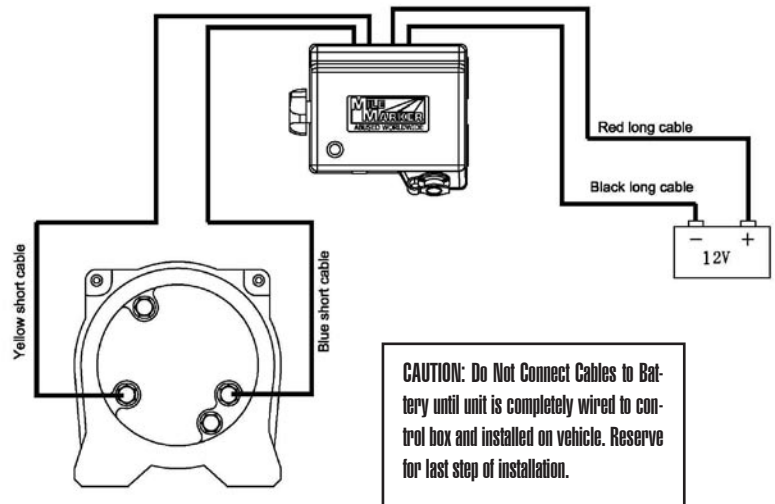
2-9: Complete Wiring Schematic: PEC8
