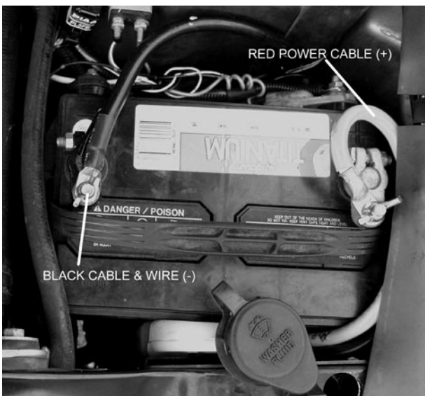
2-13: Complete Wiring to Battery
