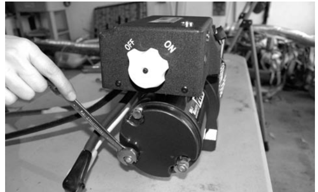
2-8: Remove Nuts and lock washer from Motor Studs (14 mm wrench)
