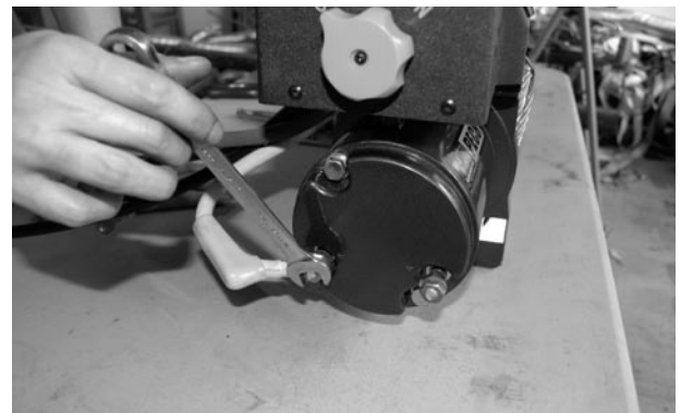
2-10: Place Cables and Replace Washer and Nut. Tighten with 14mm Wrench. Repeat for both motor studs.
